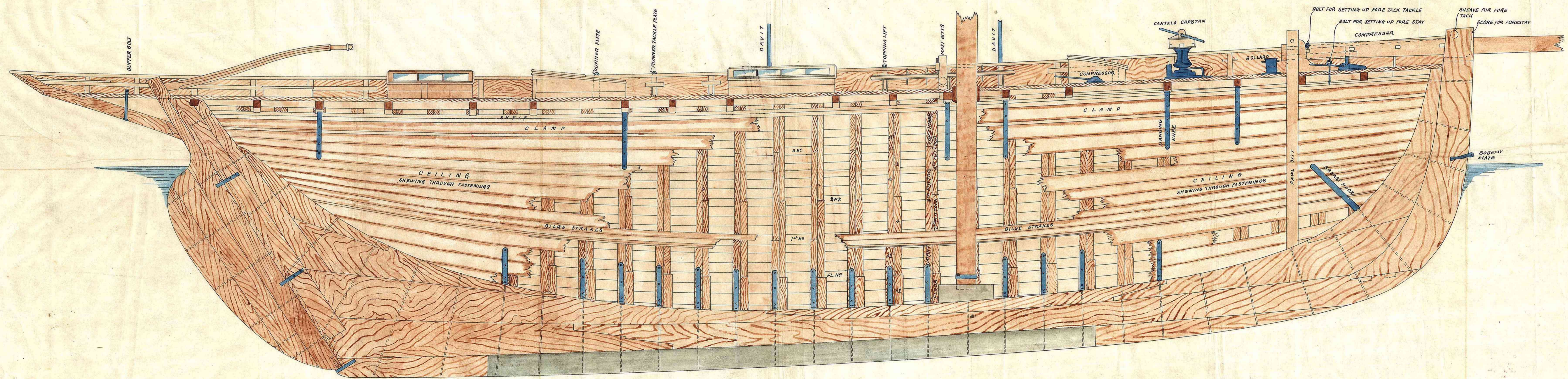
SHEER SECTION 40 TON CUTTER 1/2 INCH SCALE.
